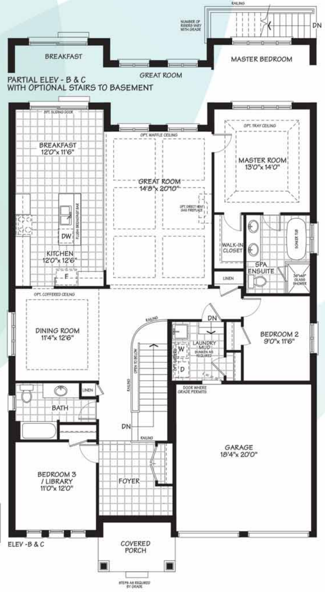
MAIN FLOOR
